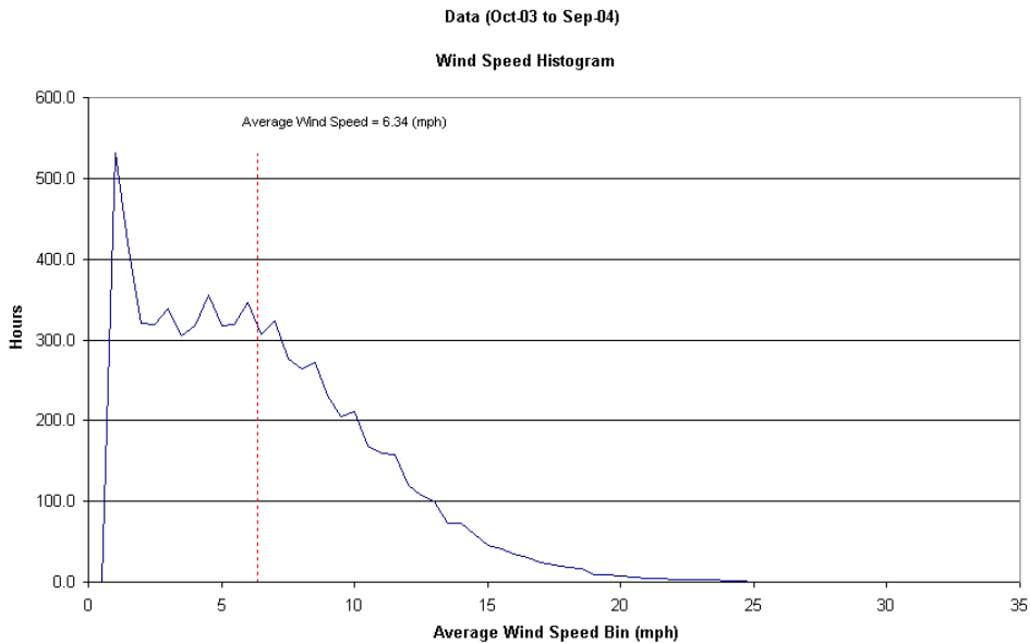
Figure 4. Wind speed frequency over the year by number of hours.
