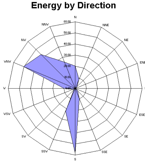
Figure 9. Energy wind rose with units in kWh/m 2 .
