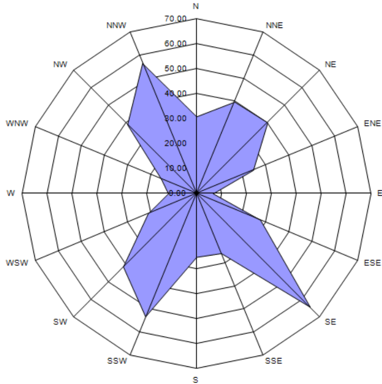
Figure E.7.9. Energy wind rose with units in kWh/m 2 .
