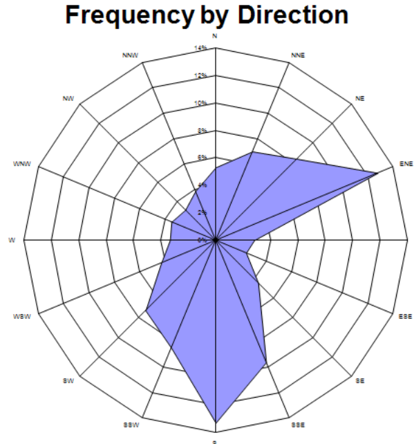
Figure E.7.8. Wind rose displaying wind direction frequency.
