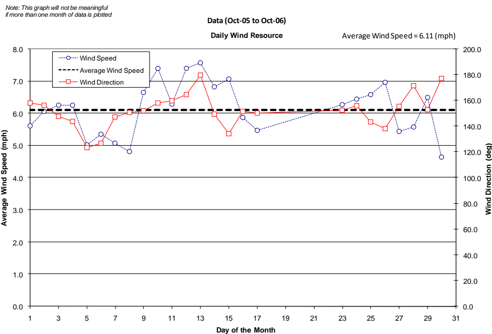
Figure E.7.6. Wind speed and direction averages by day of the month.
