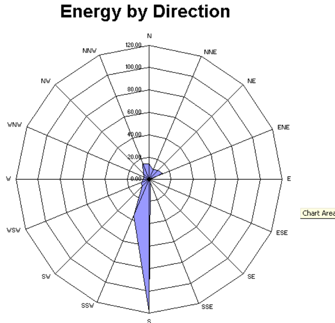
Figure 9. Energy wind rose with units in kWh/m 2 .
