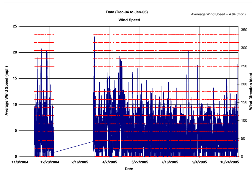
Figure 5. Wind speed and direction readings throughout the year.
