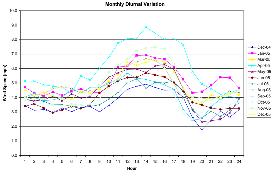
Figure 3. Average hourly wind speeds for each month.
