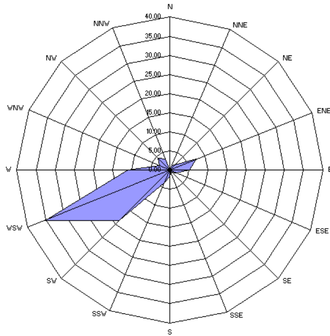
Figure 9. Energy wind rose with units in kWh/m 2 .
